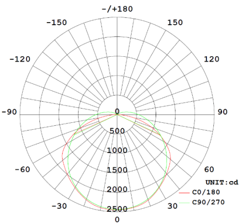
Diagram for RHE60X6FT-24 in 60W 5000K Other diagrams available on request
