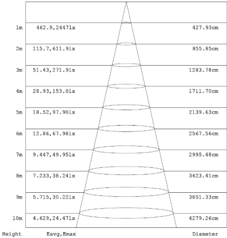
Diagram for RHE60X6FT-24 in 60W 5000K Other diagrams available on request
